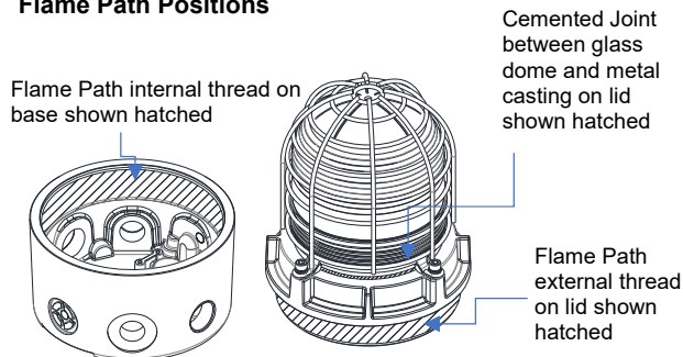
Figure 1: Flame Path.
