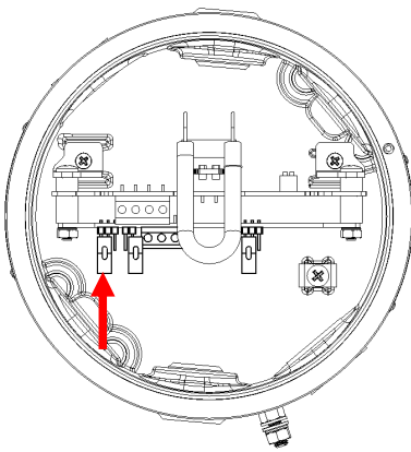
Figure 14: J2 Header pin positions – Fault Resistor (FR)
