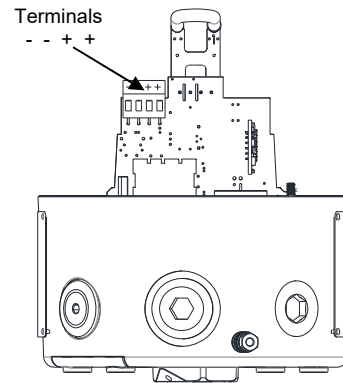
Figure 4: D1xB2XDC Terminals.
