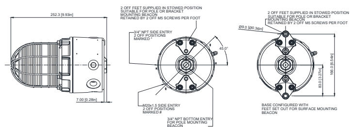
Figure 2: Fixing Location for Beacon.
