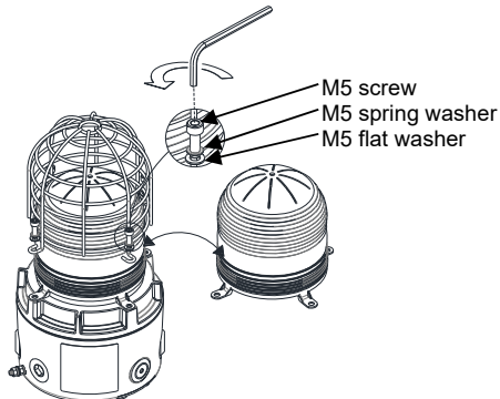
Figure 8: Replacement of beacon lens cover.
