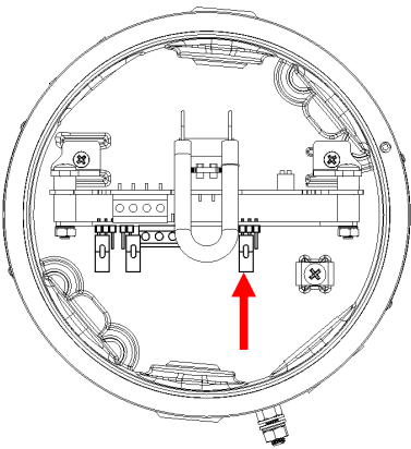
Figure 15: J7 Header pin positions – Hard Reset Function
