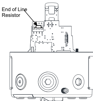
Figure 5b: End of Line Resistor Placement.
