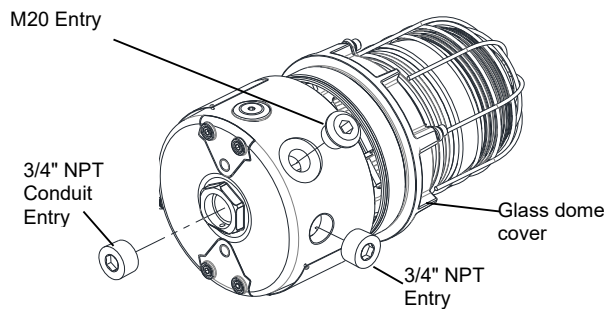
Figure 3: Accessing the Explosion Proof Enclosure.
