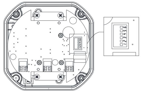
Fig. 7: DIP Switch Location
