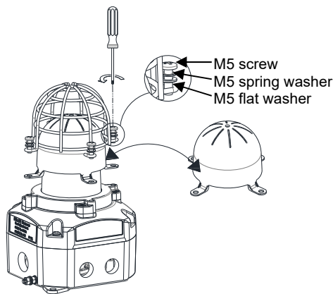
Fig. 9 Replacement of beacon lens cover
